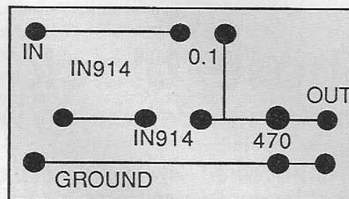
PC Board
