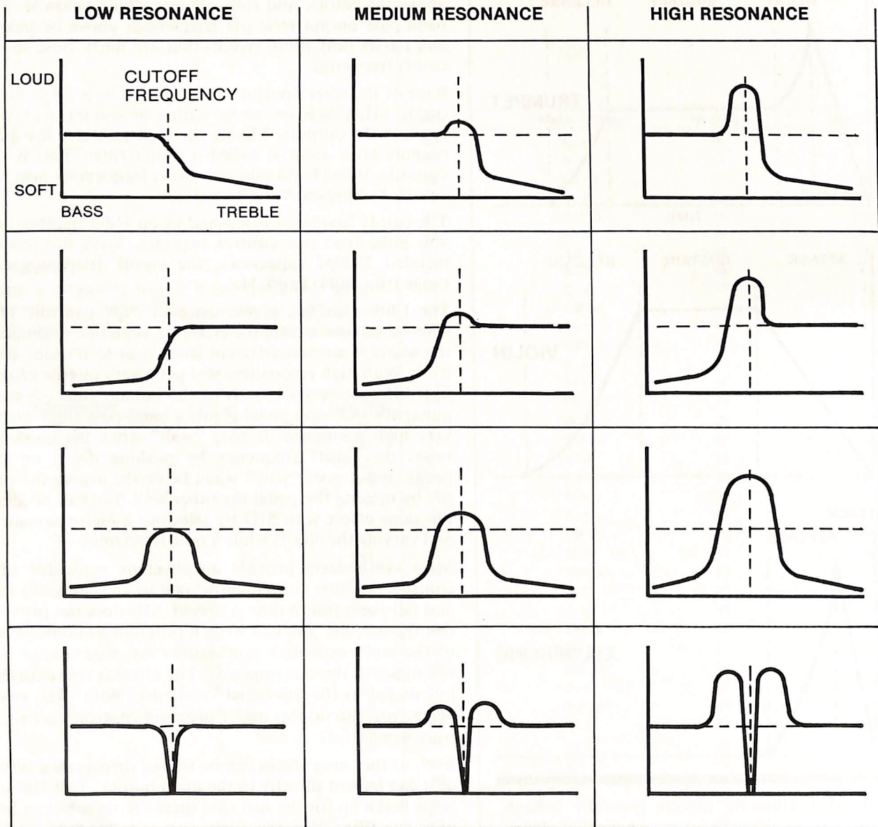
Figure 4 Some effects that SID's filter can produce.
