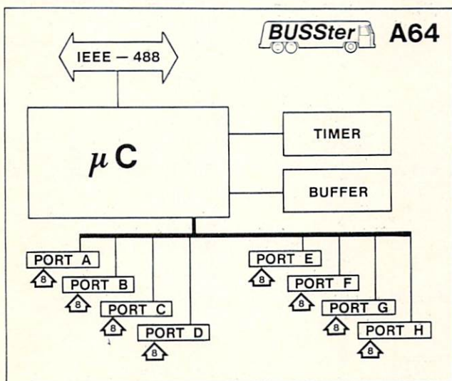
IEEE-488 64 DIGITAL CHANNEL DATA ACQUISITION INPUT MODULE
