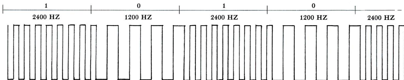
PORTION OF A SERIAL BYTE IN AUDIO FORMAT
