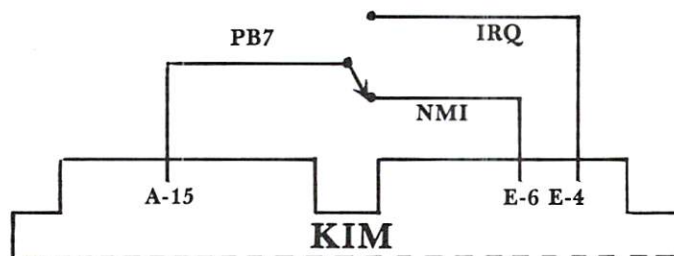
Figure 1 - Enabling the Timer Interrupt
