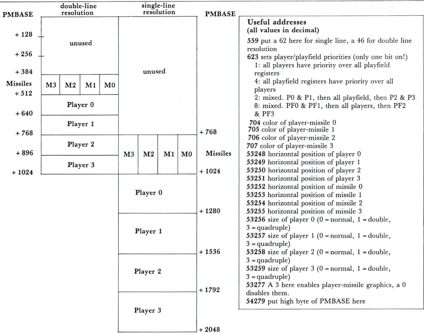
Figure 3 Player-missile graphics RAM positioning PMBASE must be on 1K boundary for double-line resolution, 2K boundary for single-line resolution
