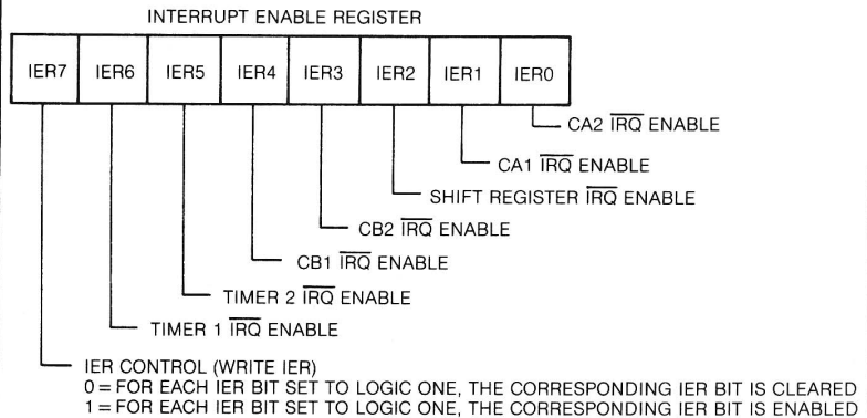
Figure 6: A diagram of the 6522's Interrupt Enable Register (IER).
