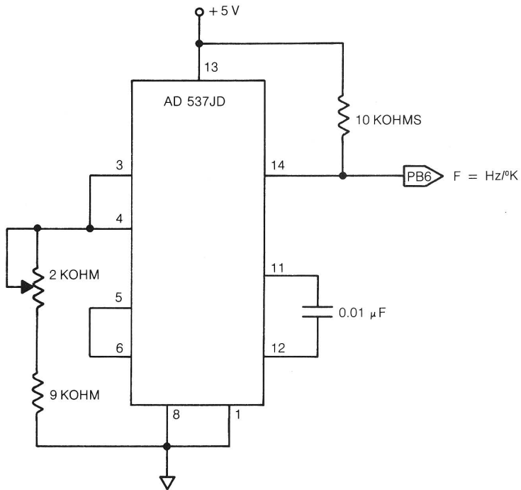
Figure 9: A Temperature-to-Frequency Converter
