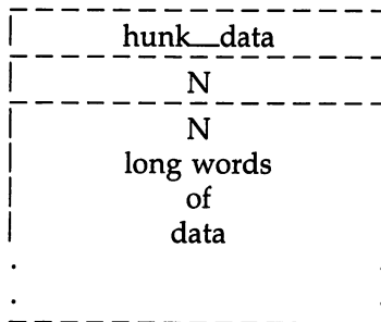
Figure 1-D: hunk_data (1002/3EA)
