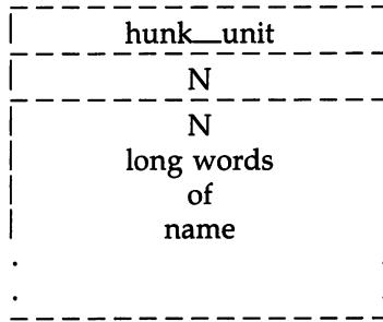
Figure 2-A: hunk__unit (999/3E7)
