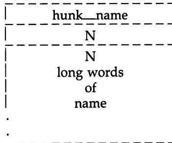
Figure 2-B: hunk__name (1000/3E8)
