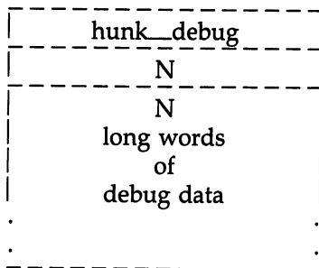
Figure 2-K: hunk__debug (1009/3F1)
