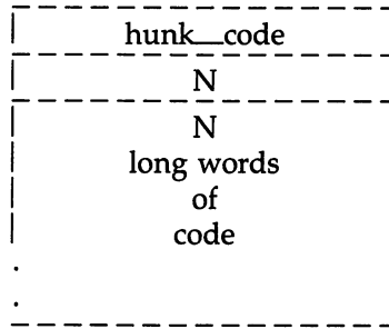
Figure 1-C: hunk_code (1001/3E9)
