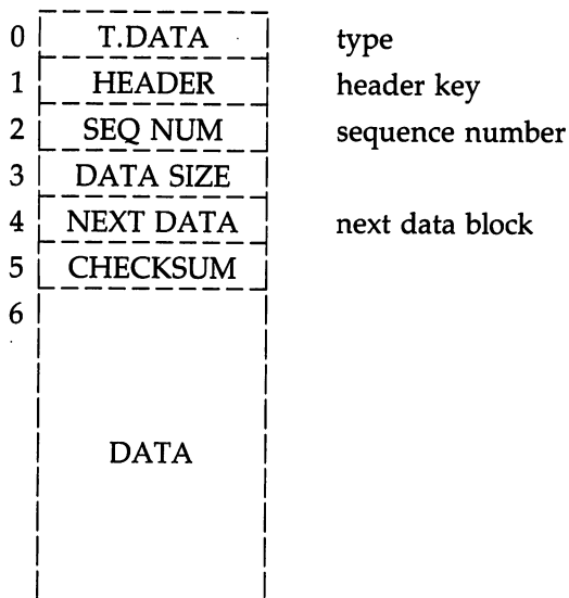
Figure 1-E: Data Block
