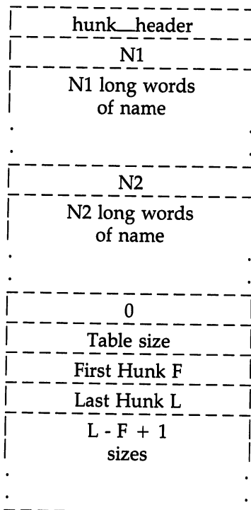
Figure 2-L: hunk_header (1011/3F3)
