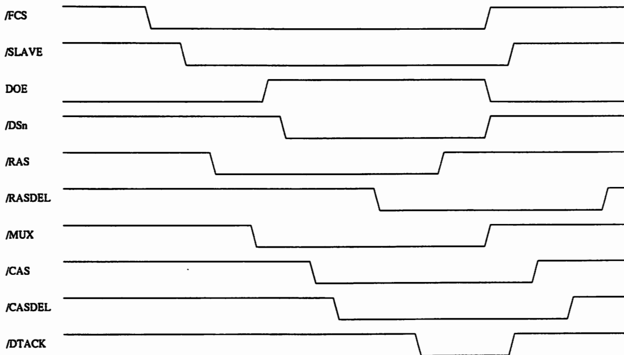
Figure 3-3: Memory Access
