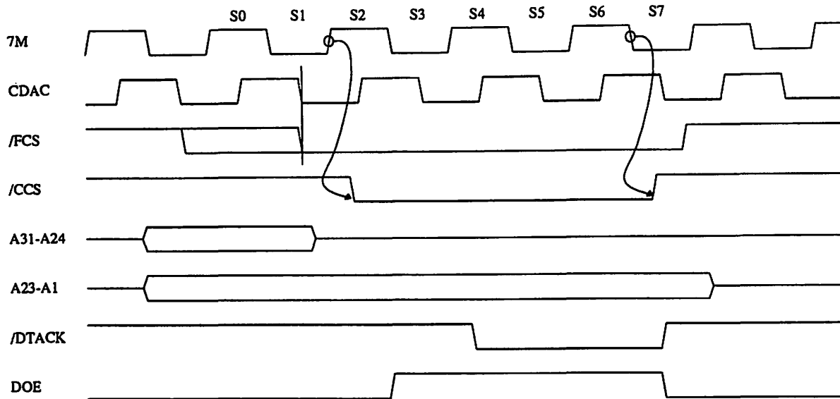
Figure 3-5: Zorro II Within Zorro III
