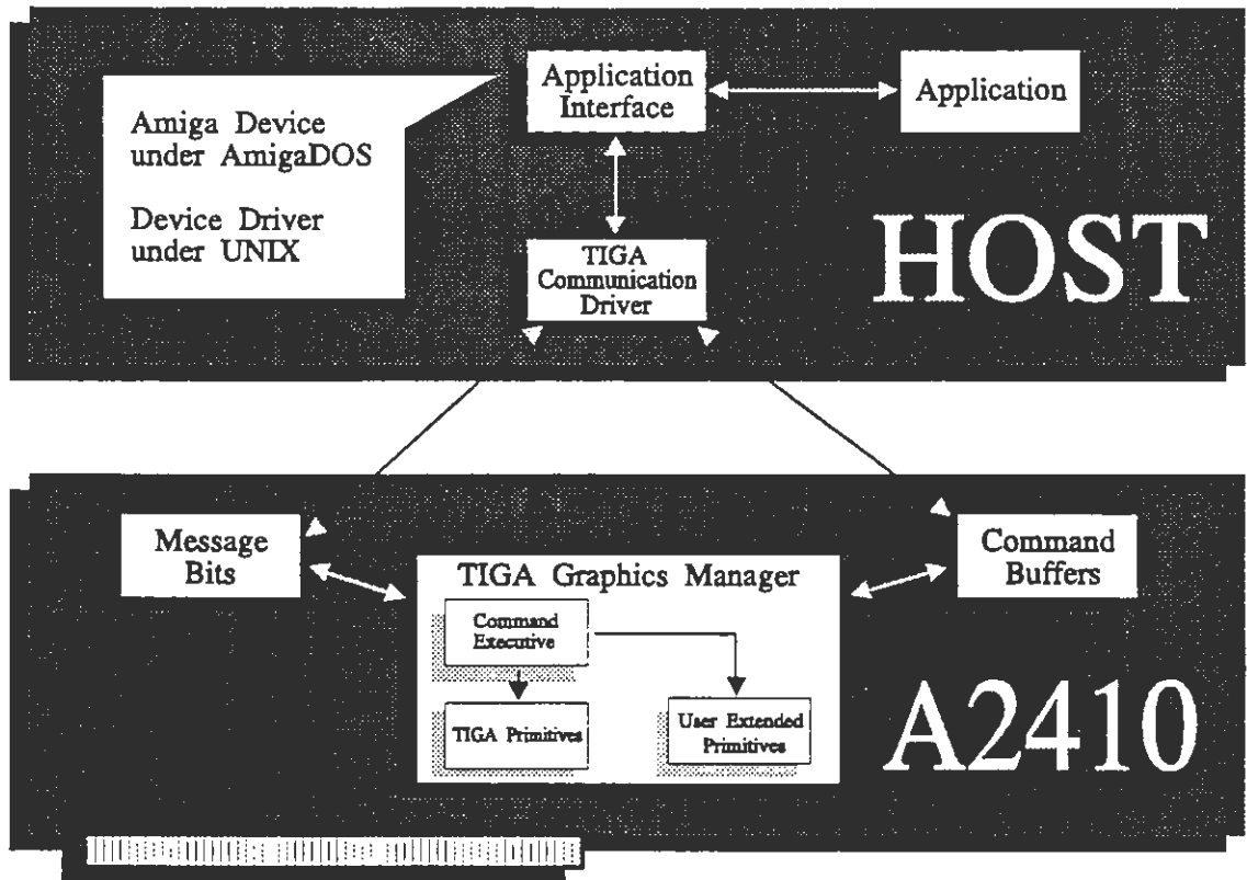
Figure 5: Texas Instruments Graphics Architecture (TIGA) Block Diagram
