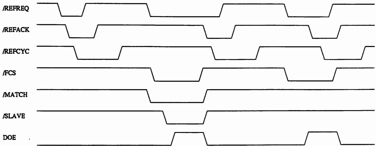
Figure 3-1: Refresh Arbitration
