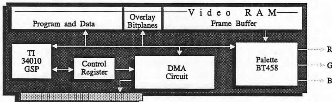
Figure 1: Block Diagram of the A2410 High Resolution Color Graphics Card
