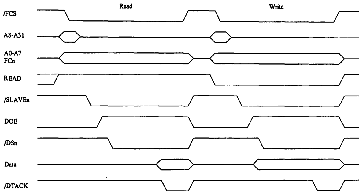
Figure 3-1: Basic Zorro III Cycles
