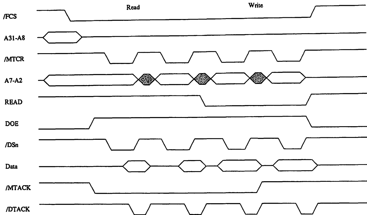
Figure 3-2: Multiple Transfer Cycles
