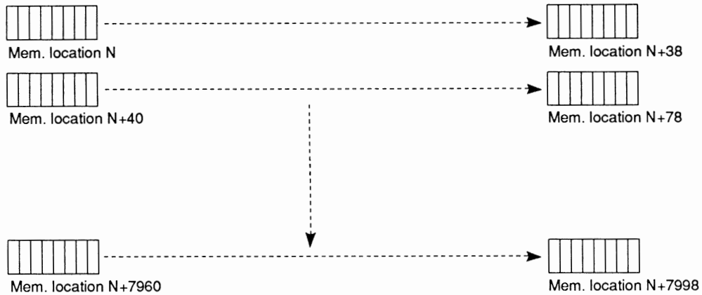
Figure 3-7: Memory Organization for a Basic Bitplane
