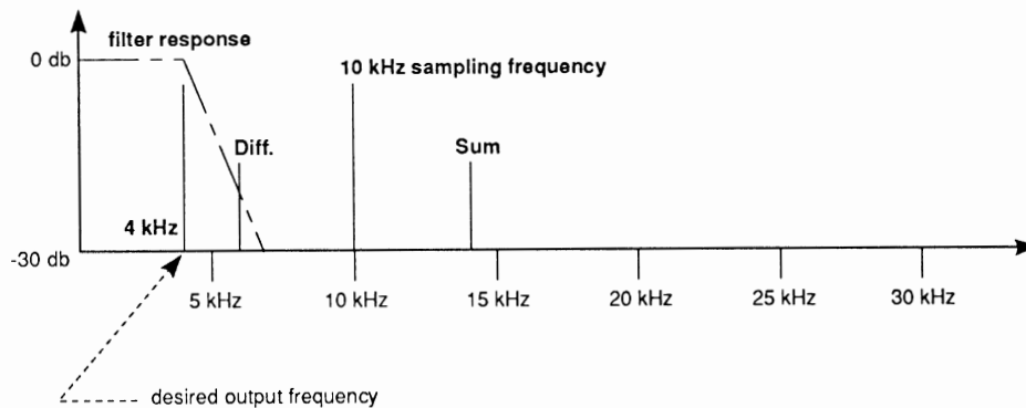
Figure 5-7: Some Aliasing Distortion
