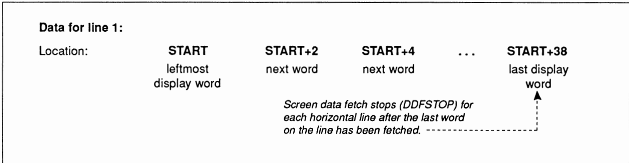
Figure 3-15: Data Fetch for the First Line When Modulo = 40
