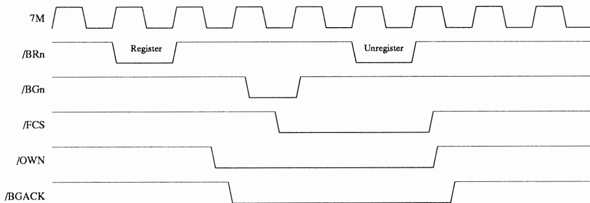
Figure K-7: Zorro III Bus Arbitration
