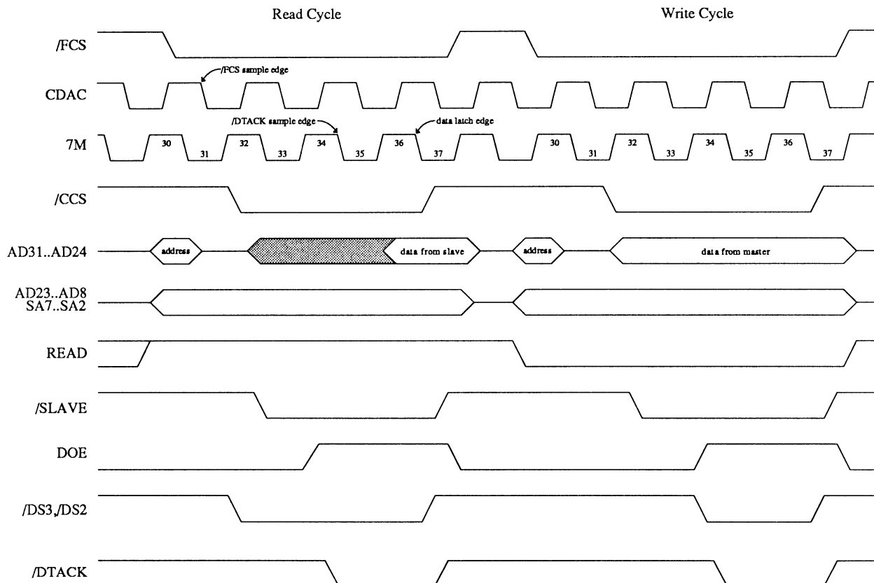
Figure K-9: Zorro II Within Zorro III
