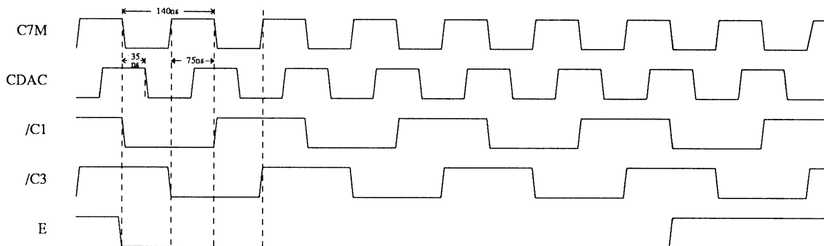
Figure K-3: Expansion Bus Clocks
