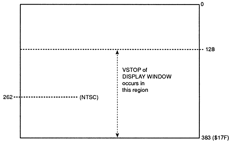
Figure 3-22: Display Window Vertical Stopping Position
