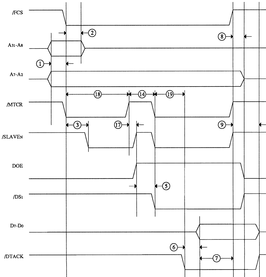
Figure K-13: Quick Interrupt Cycle Timing
