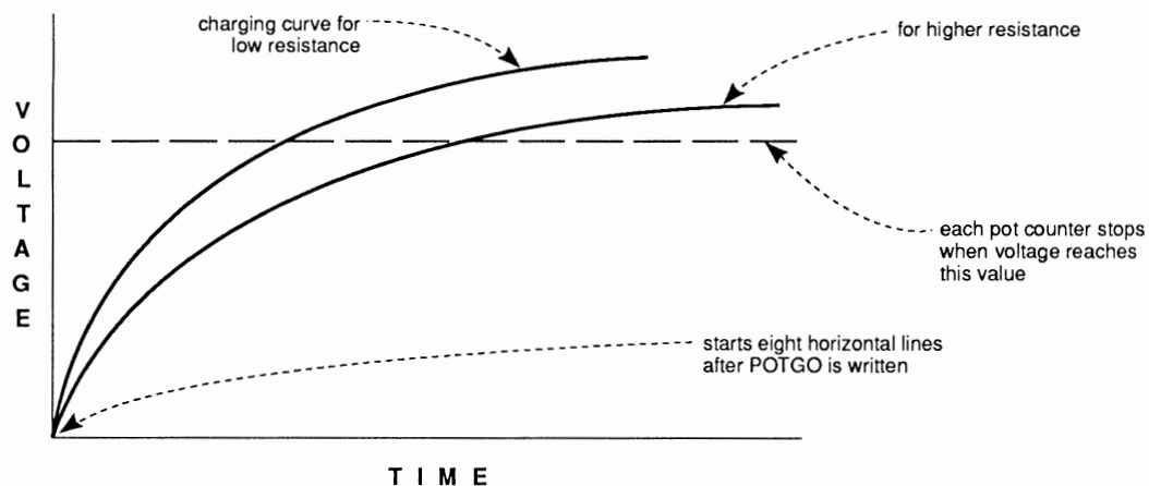
Figure 8-5: Effects of Resistance on Charging Rate
