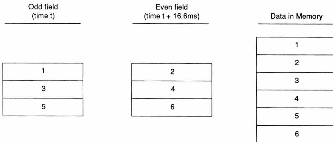
Figure 2-1: Interlaced Bitplane in RAM
