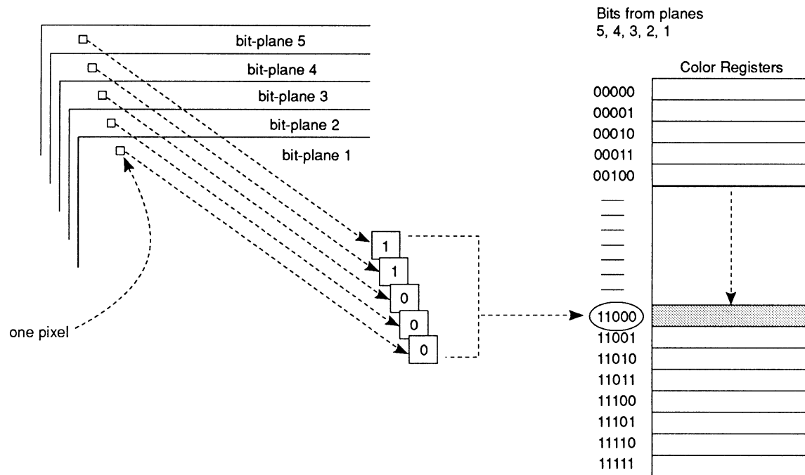
Figure 3-3: How Bitplanes Select a Color
