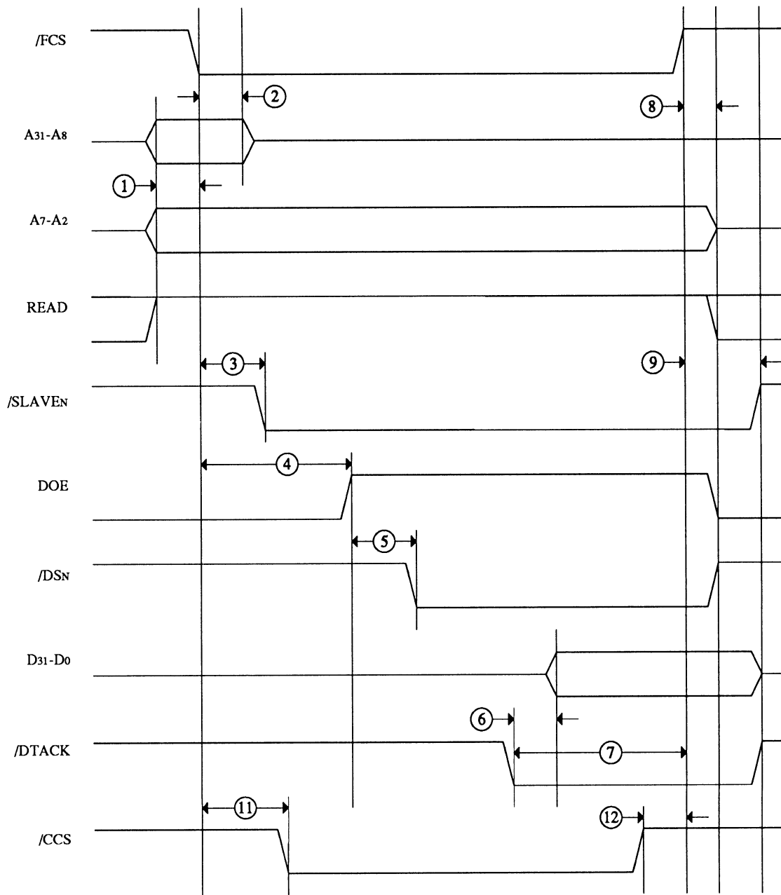
Figure K-10: Read Cycle Timing
