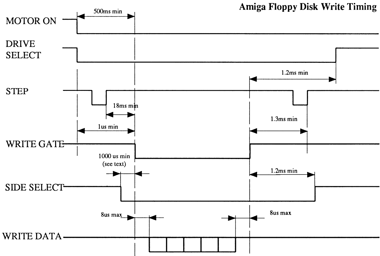
Figure 1-7: Chinon Timing Diagram
