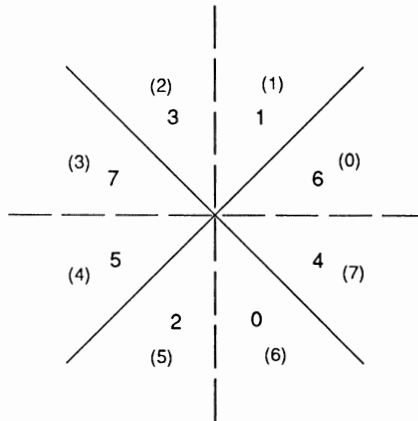
Figure 6-8: Octants for Line Drawing
