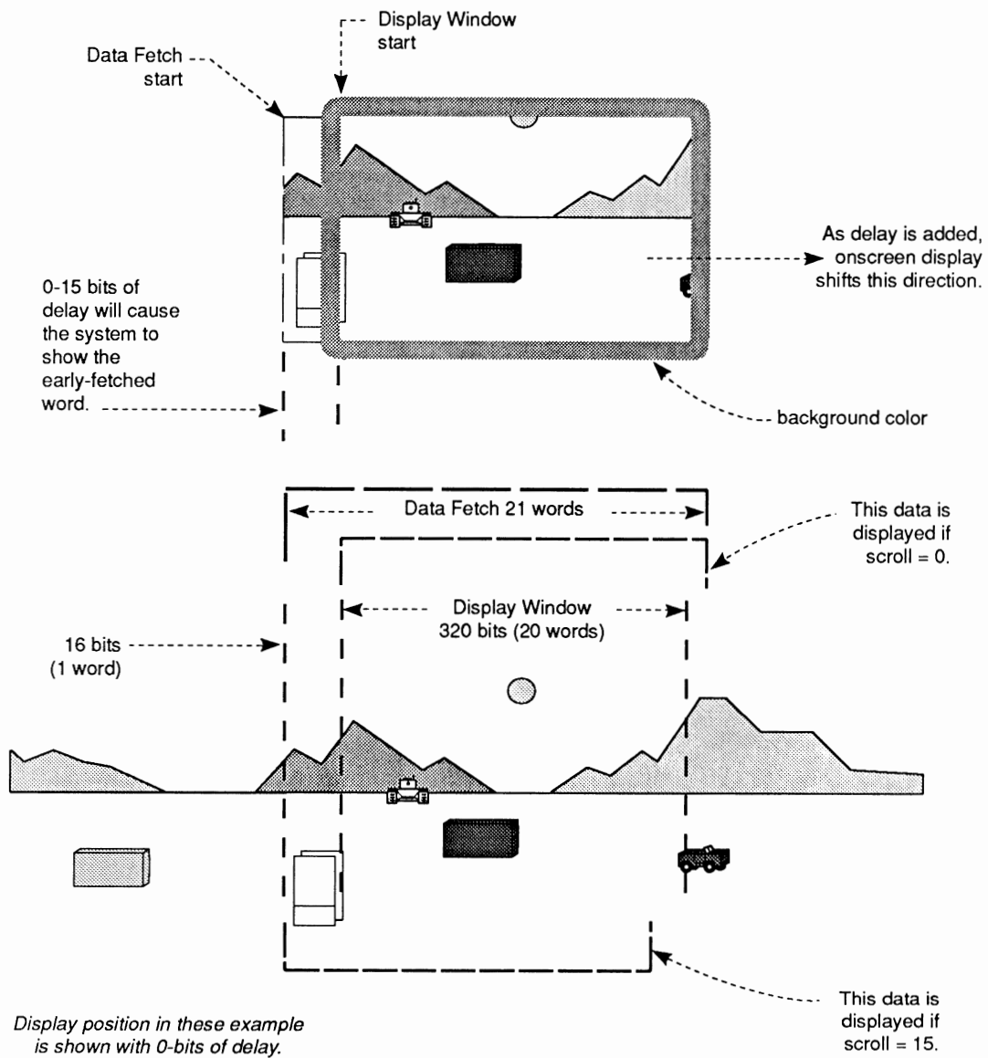
Figure 3-24: Horizontal Scrolling
