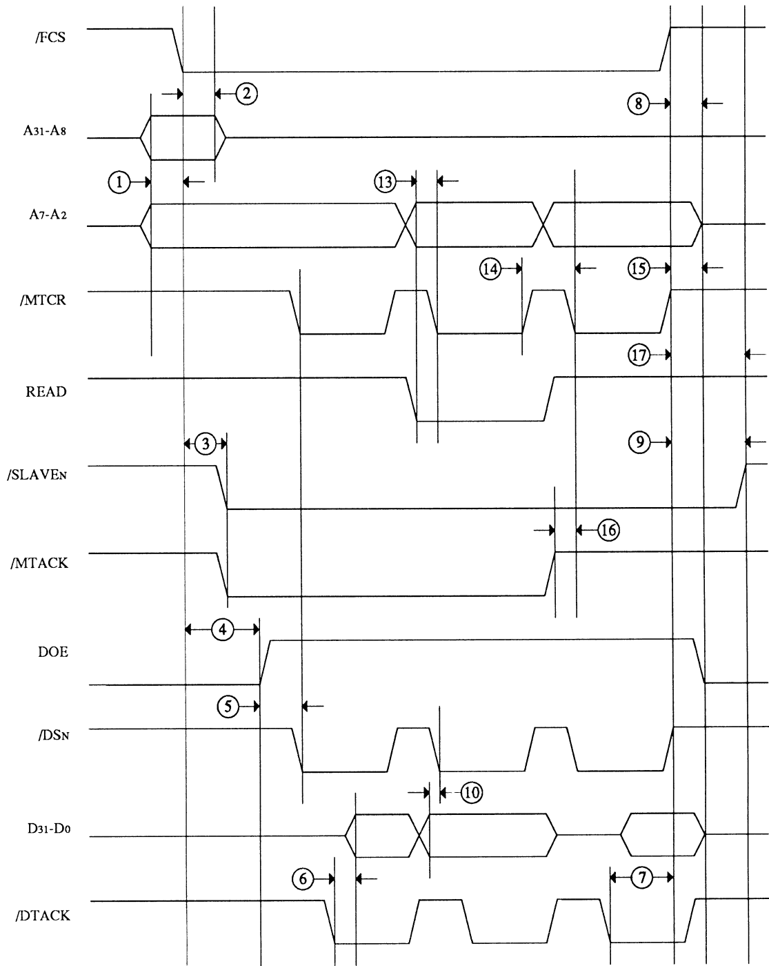
Figure K-12: Multiple Transfer Cycle Timing
