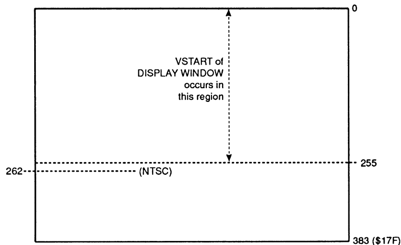
Figure 3-20: Display Window Vertical Starting Position
