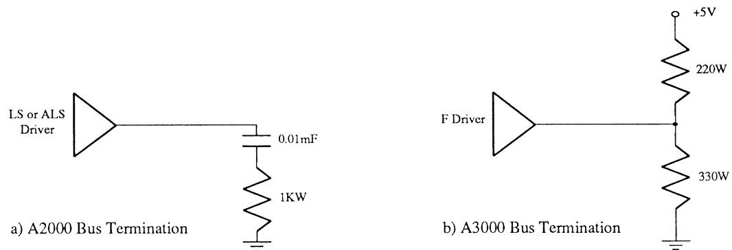
Figure K-2: A2000 vs. A3000 Bus Termination
