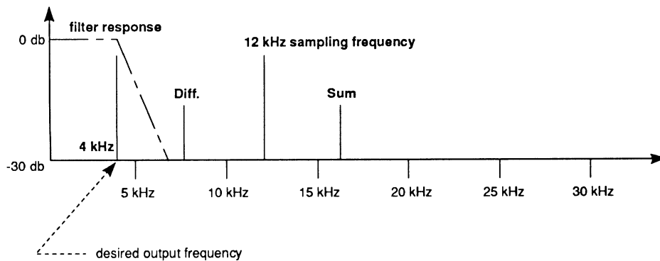
Figure 5-6: Noise-free Output (No Aliasing Distortion)
