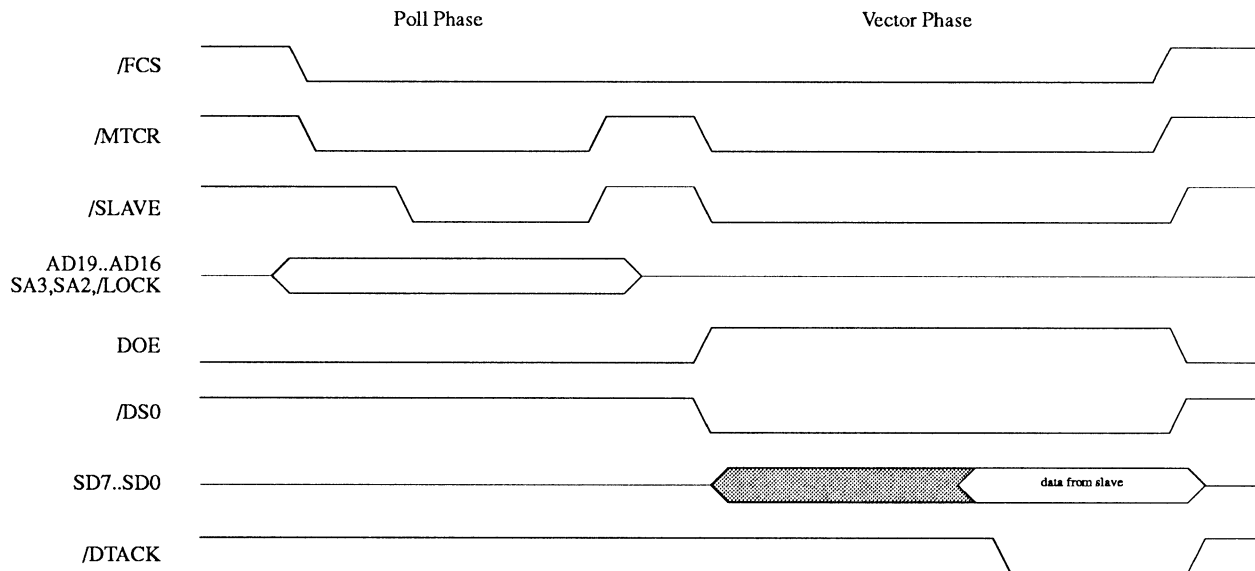
Figure K-8: Interrupt Vector Cycle
