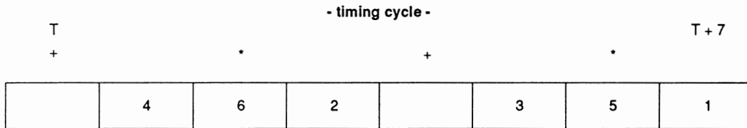
Figure 6-11: Time Slots Used by a Six Bitplane Display
