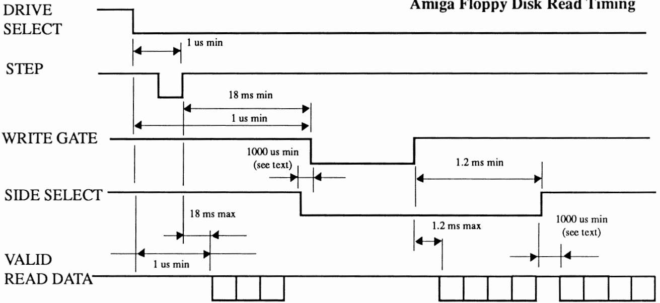
Figure 8-8: Chinon Timing Diagram (cont.)
