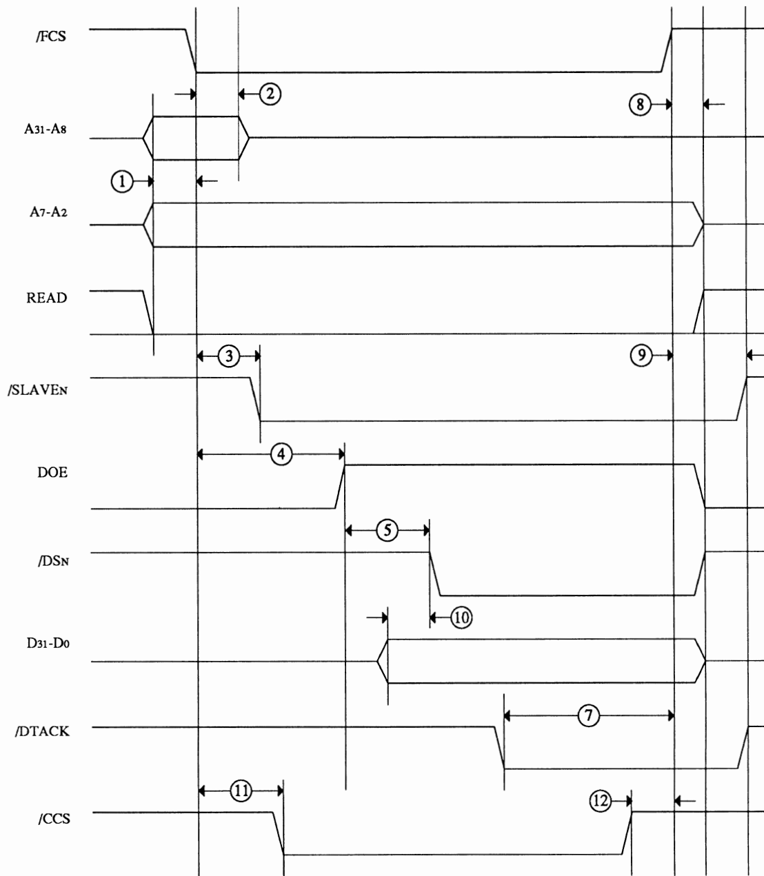
Figure K-11: Write Cycle Timing
