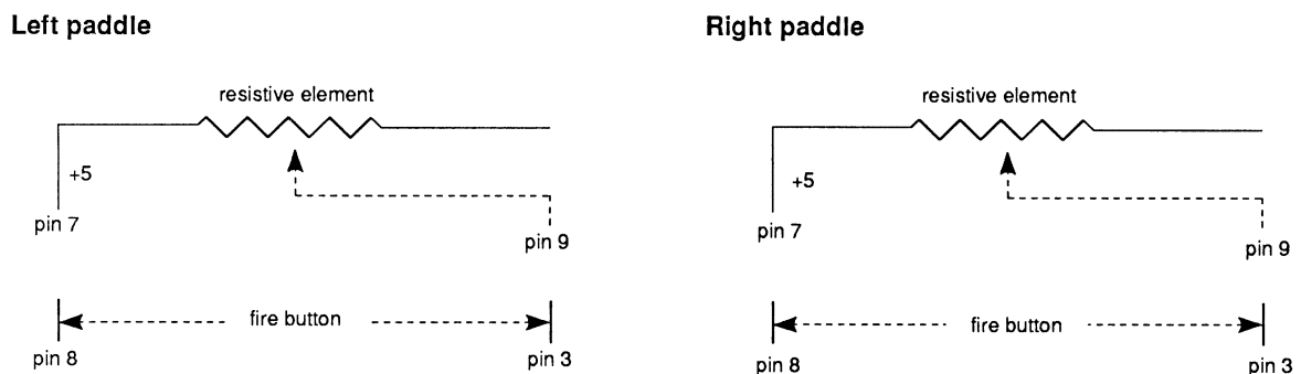
Figure 8-4: Typical Paddle Wiring Diagram
