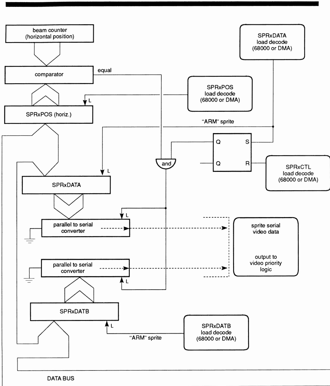
Figure 4-13: Sprite Control Circuitry
