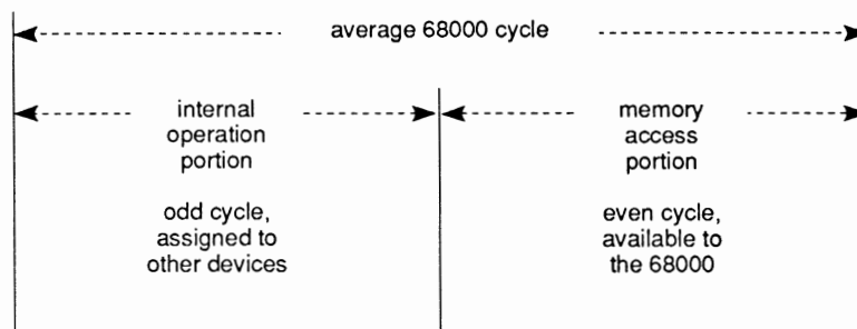
Figure 6-10: Normal 68000 Cycle
