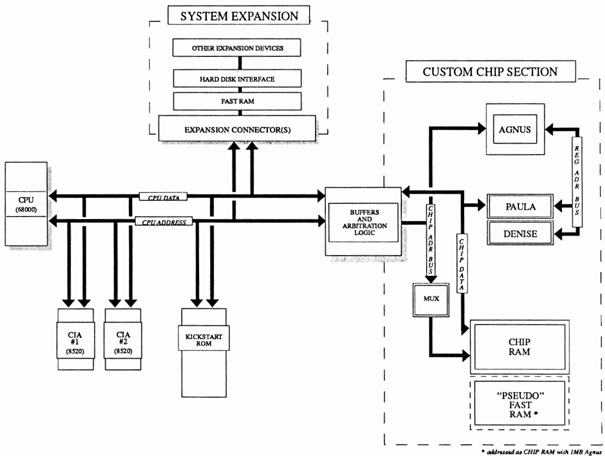
Figure 1-1: Block Diagram for the Amiga Computer Family
