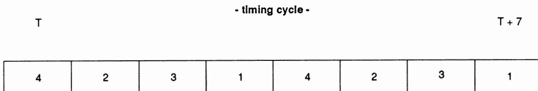
Figure 6-12: Time Slots Used by a High Resolution Display
