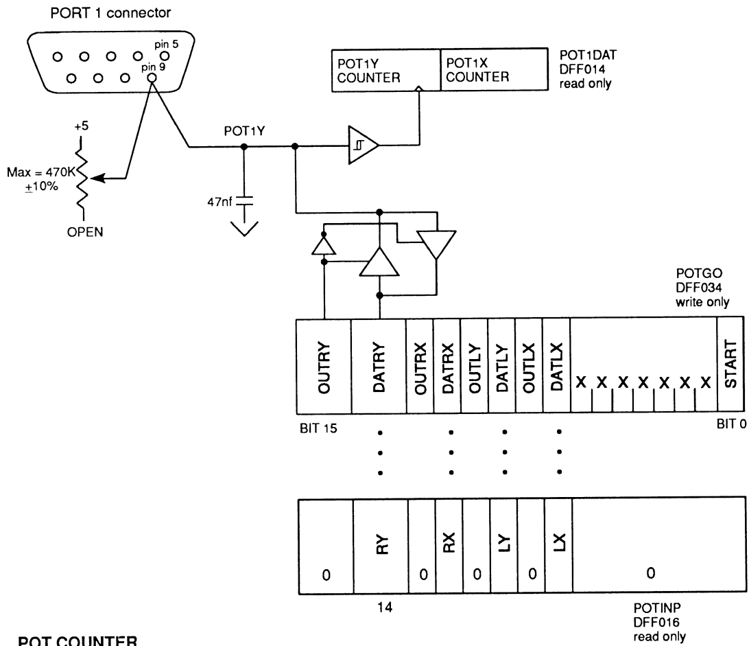
Figure 8-6: Potentiometer Charging Circuit
