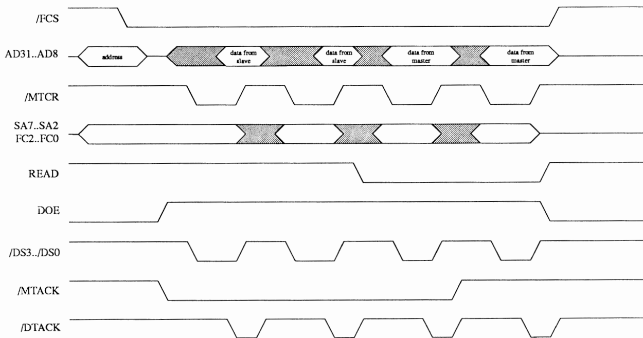
Figure K-6: Multiple Transfer Cycles
