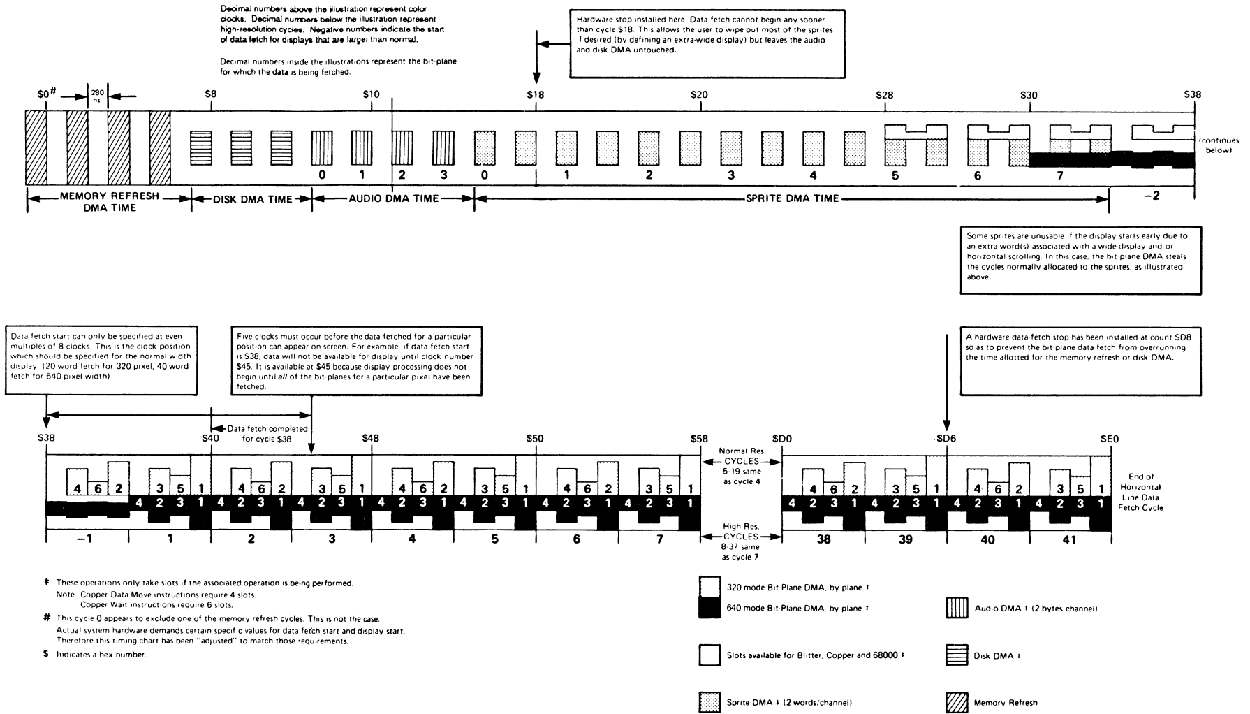
Figure 6-9: DMA Time Slot Allocation
