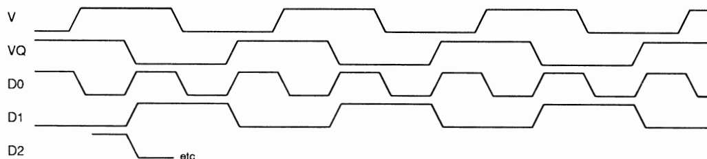
Figure 8-2: Mouse Quadrature
