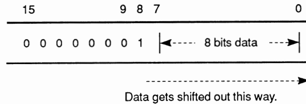
Figure 8-12: Ending Appearance of Shift Register
