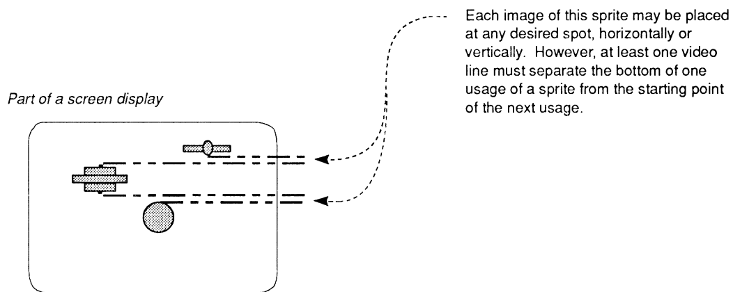
Figure 4-9: Typical Example of Sprite Reuse
