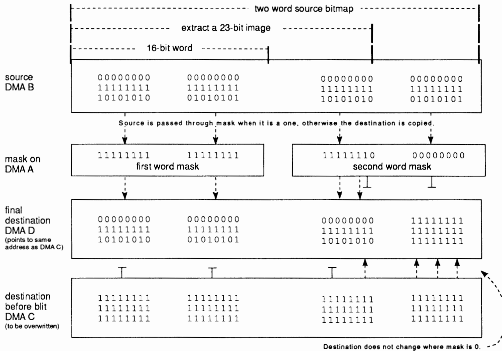
Figure 6-4: Extracting a Range of Columns
