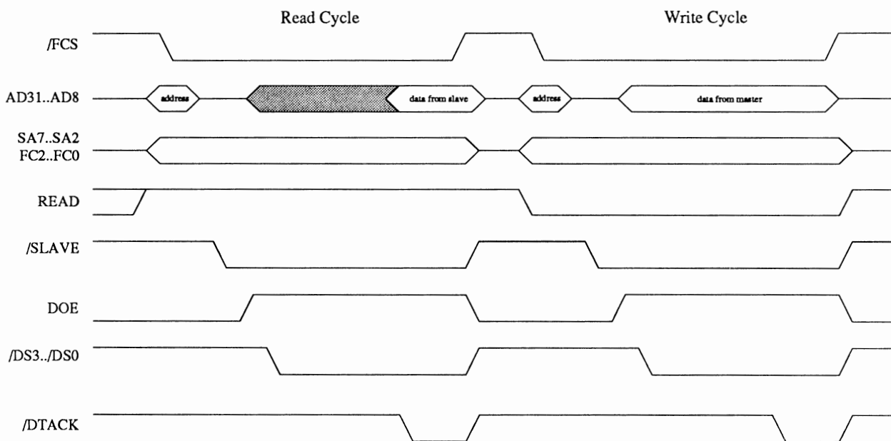
Figure K-5: Basic Zorro III Cycles
