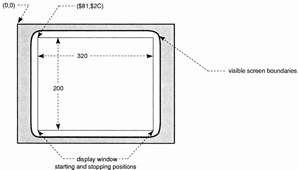
Figure 3-9: Positioning the On-screen Display
