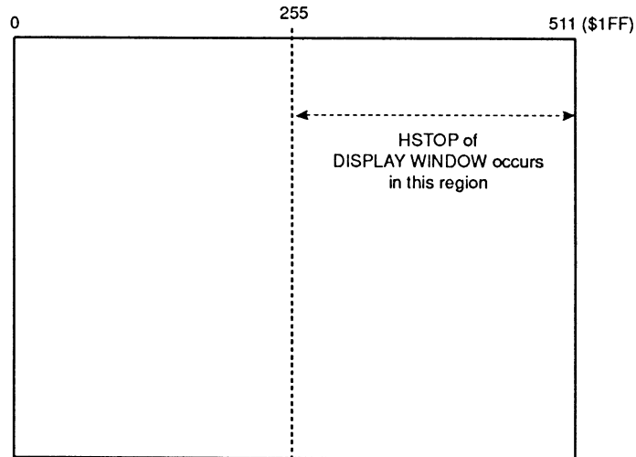
Figure 3-21: Display Window Horizontal Stopping Position
