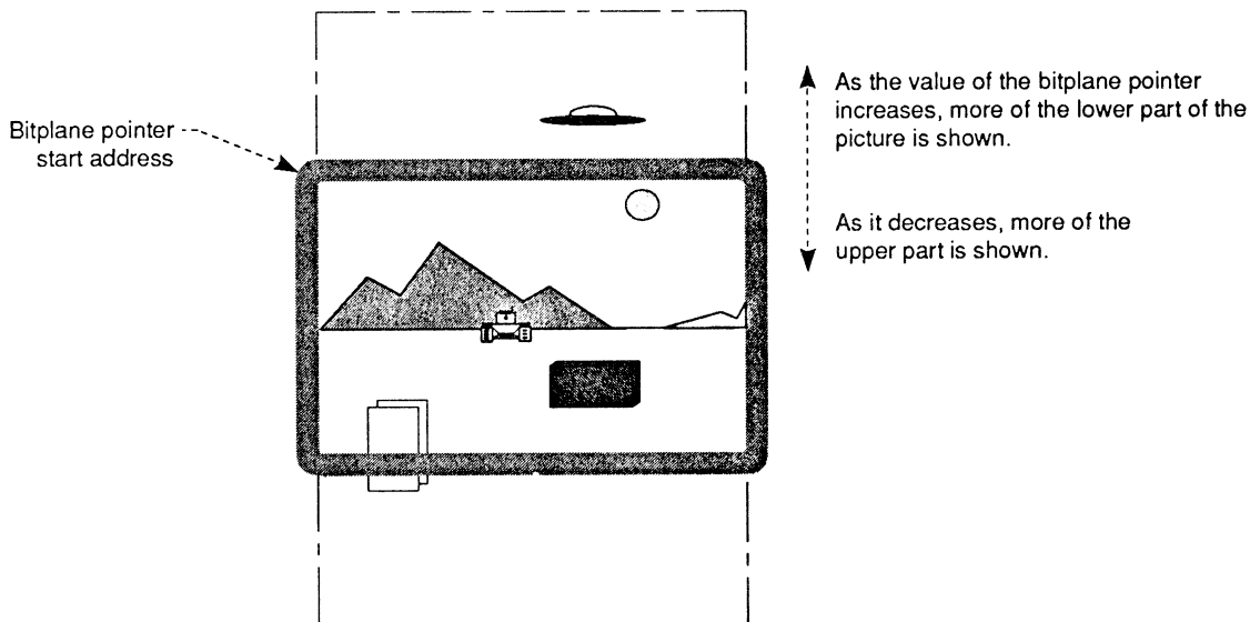
Figure 3-23: Vertical Scrolling
