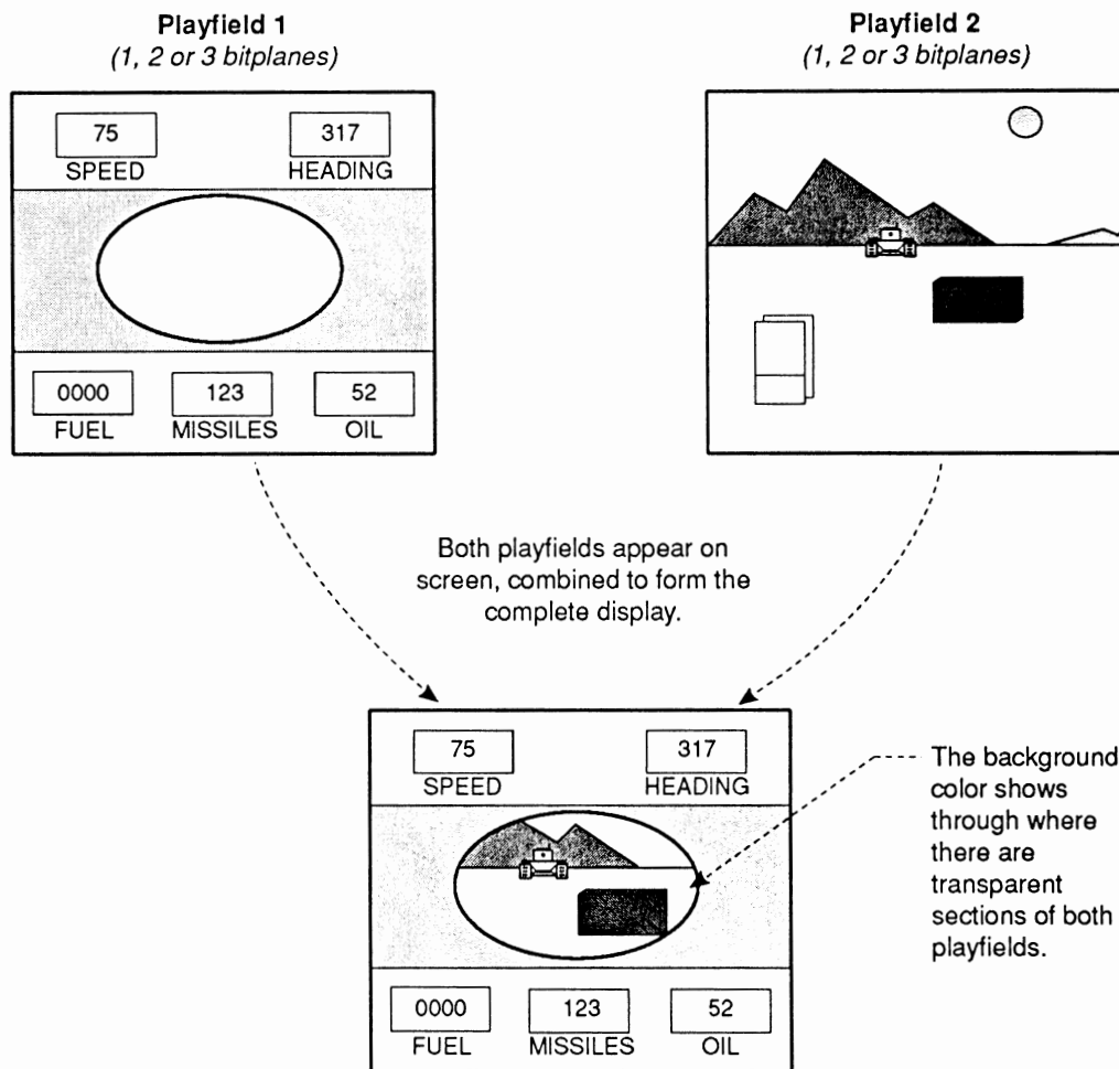
Figure 3-12: A Dual-playfield Display
