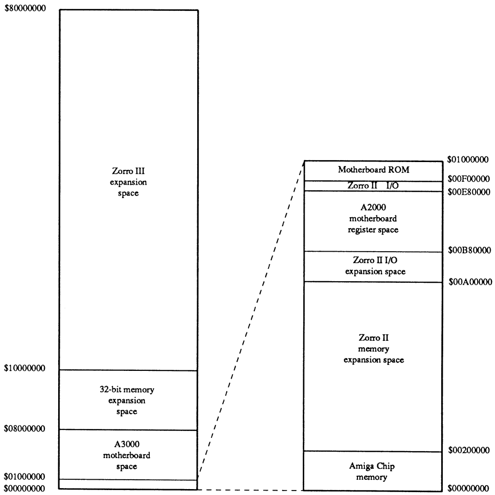
Figure K-1: Expansion Memory Map
