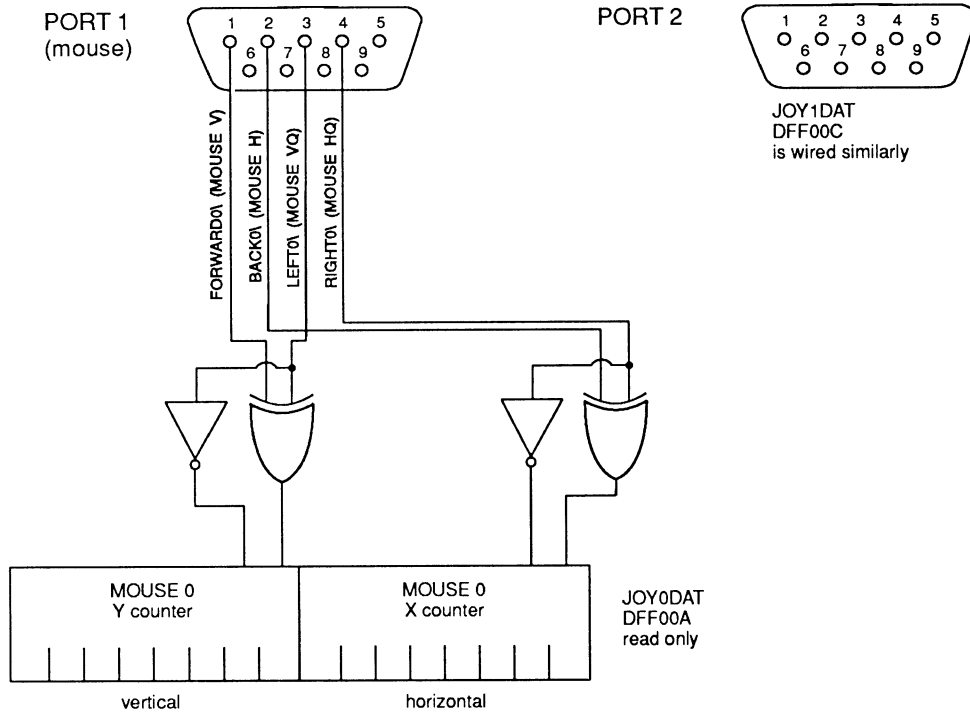
Figure 8-3: Joystick to Counter Connections
