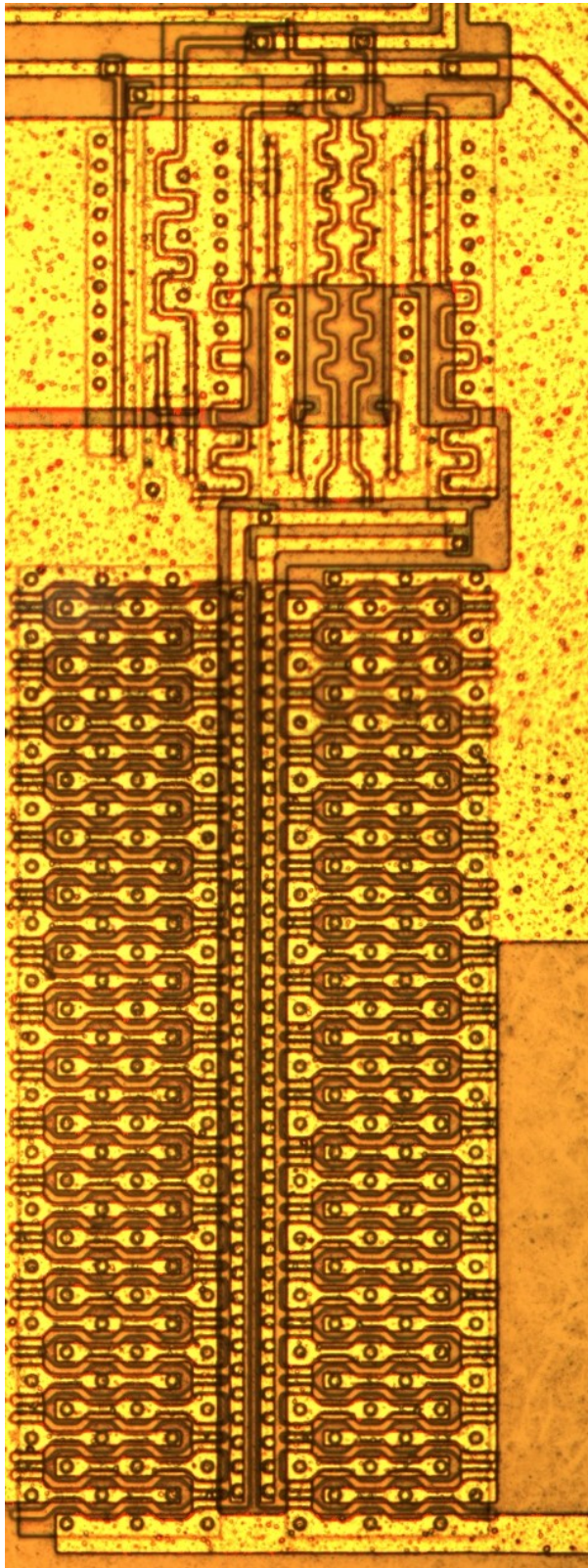
Figure 4.22: Die photograph of the output stage
