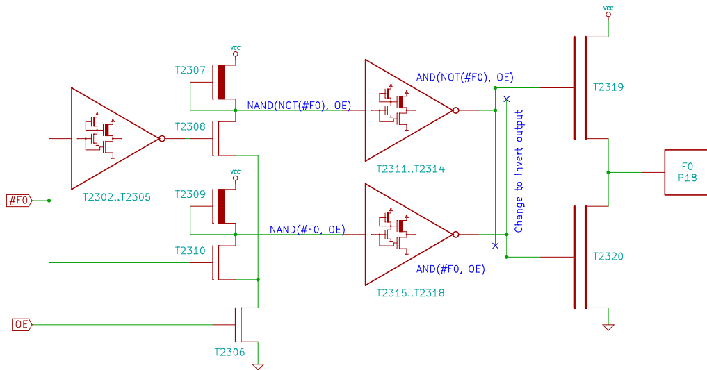
Figure 4.24: Schematic of the output stage
