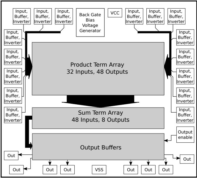
Figure 4.7: Block Diagram of the CSG PLA
