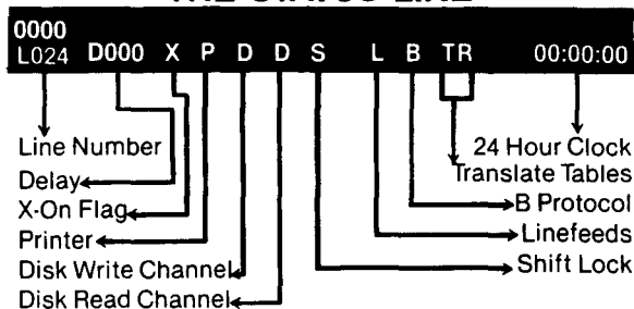
FIGURE 4-1 THE STATUS LINE
