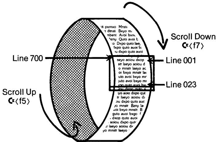
FIGURE 4-2 VIRTUAL SCREEN SCROLLING
